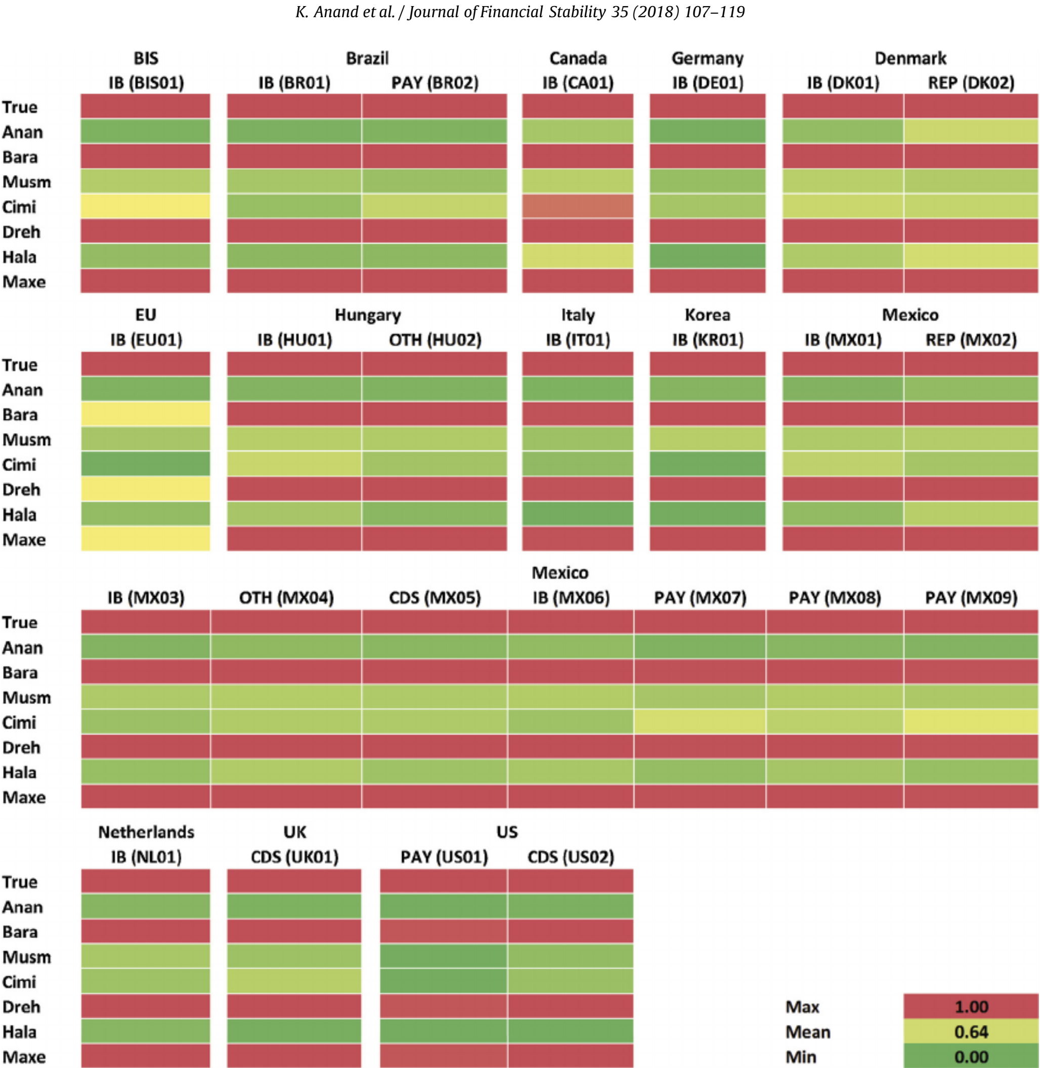
Fig. 4. Percentage of true-links. Note: true-links are defined as the percentage of realized links also found in the reconstructed network. The cells are shaded according to the relative true-links ranging from green to red. (For interpretation of the references to color in this figure legend, the reader is referred to the web version of this article.)
